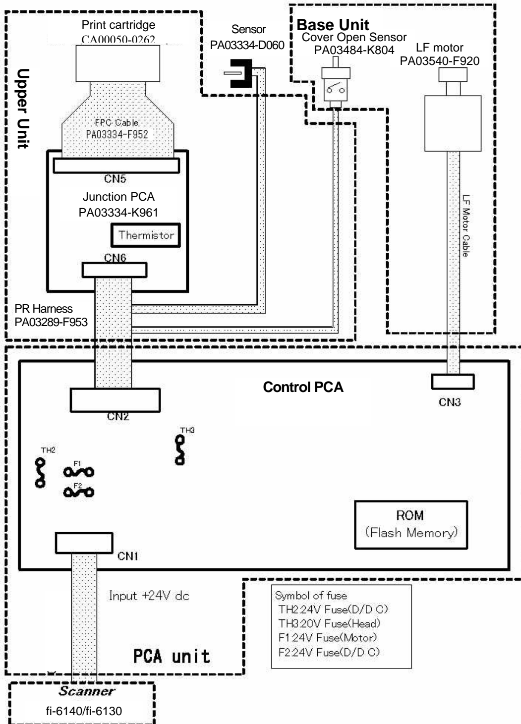
Electric Component Block Diagram
